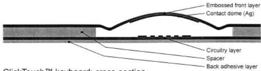
ClickTouch™ keyboard: cross-section
