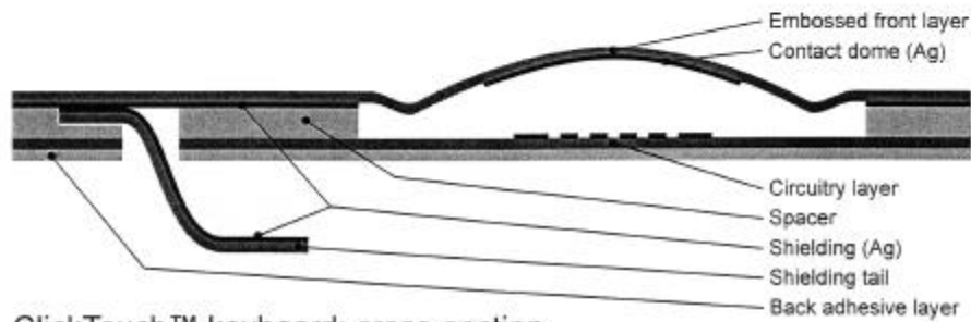
ClickTouch™ keyboard: cross-section 3-layer shielding
