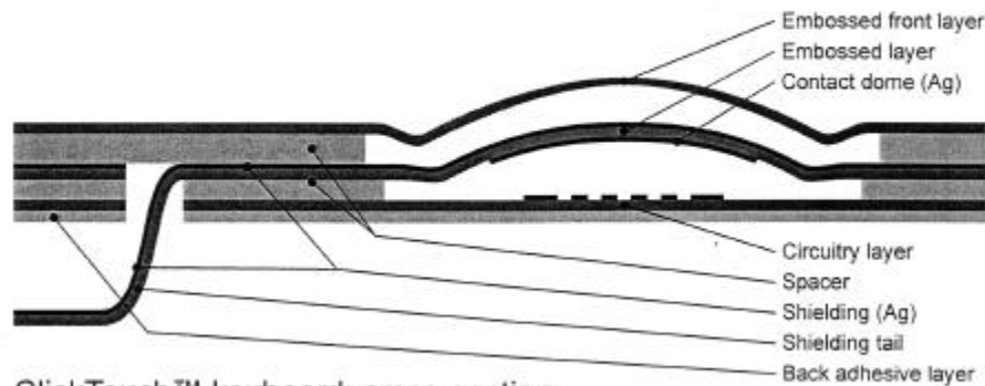
ClickTouch™ keyboard: cross-section 5-layer shielding
